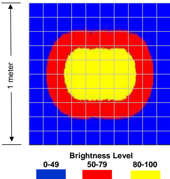
Brightness Distribution Measured at 1m
